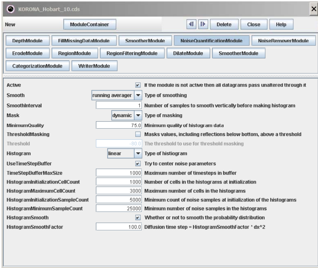
Figure 2. Setup of the LSSS real-time system (KORONA).
